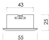
Lamphead details.
