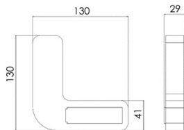
FLE31/32 CB module details.
